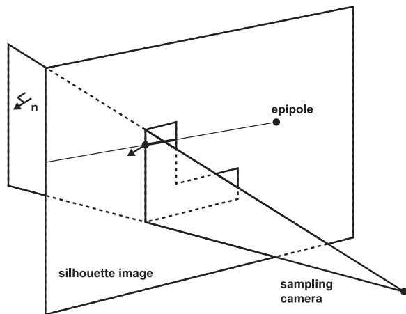
Figure 8: A silhouette edge combined with the center of projection define a plane. Visual hull interval endpoints defined by that edge have the same normal as the plane.
